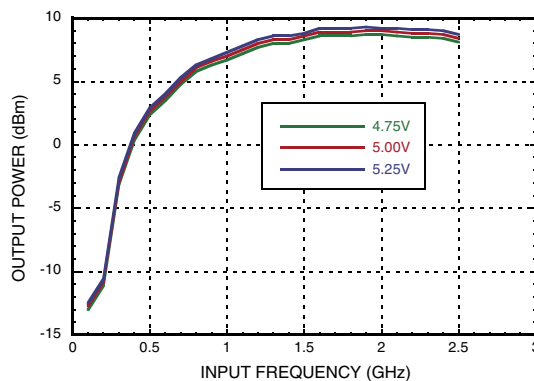
Pout Divide-by-4 vs. Supply Voltage [1] , (Differential)
